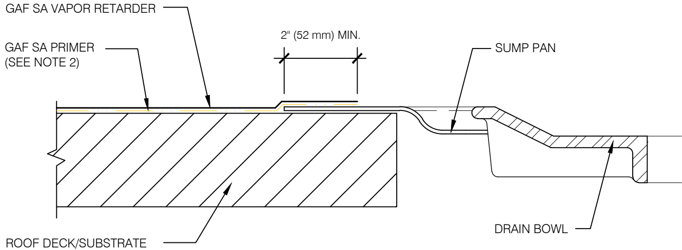
ROOF DRAIN WITH SUMP PAN
